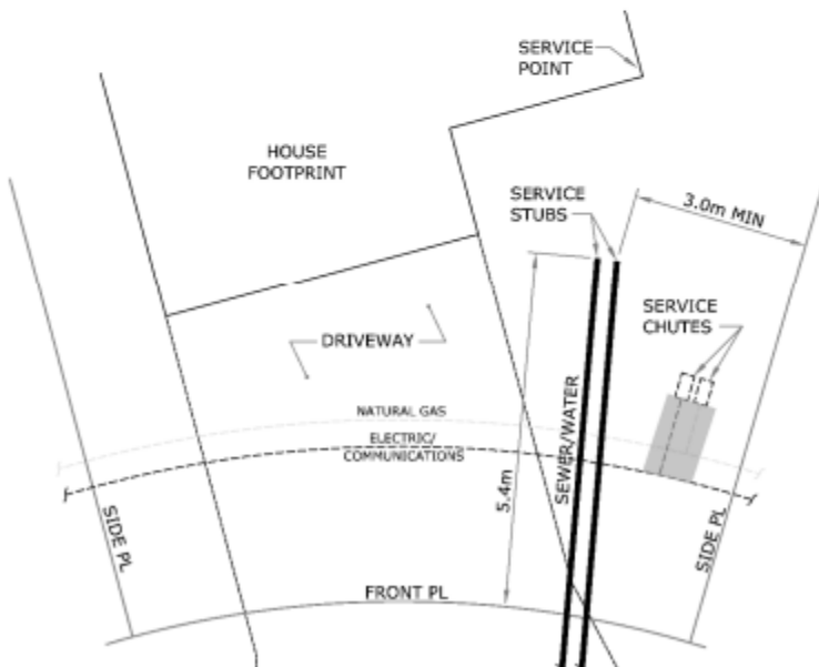
FIGURE 23 - TYPICAL SERVICE STUB LOCATION - PIE LOT MAIN TRENCH ON EASEMENT
