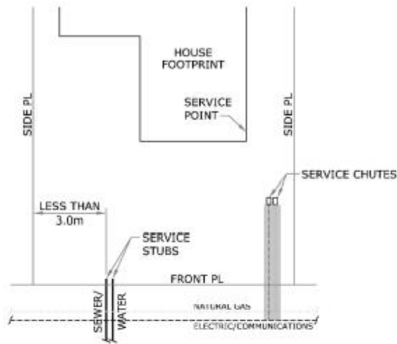
FIGURE 28 - ALTERNATE SERVICE STUB LOCATION MAIN TRENCH ON RIGHT OF WAY
