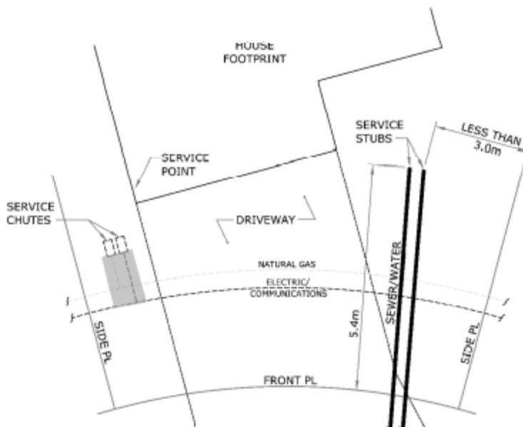
FIGURE 25 - ALTERNATE SERVICE STUB LOCATION - PIE LOT MAIN TRENCH ON EASEMENT
