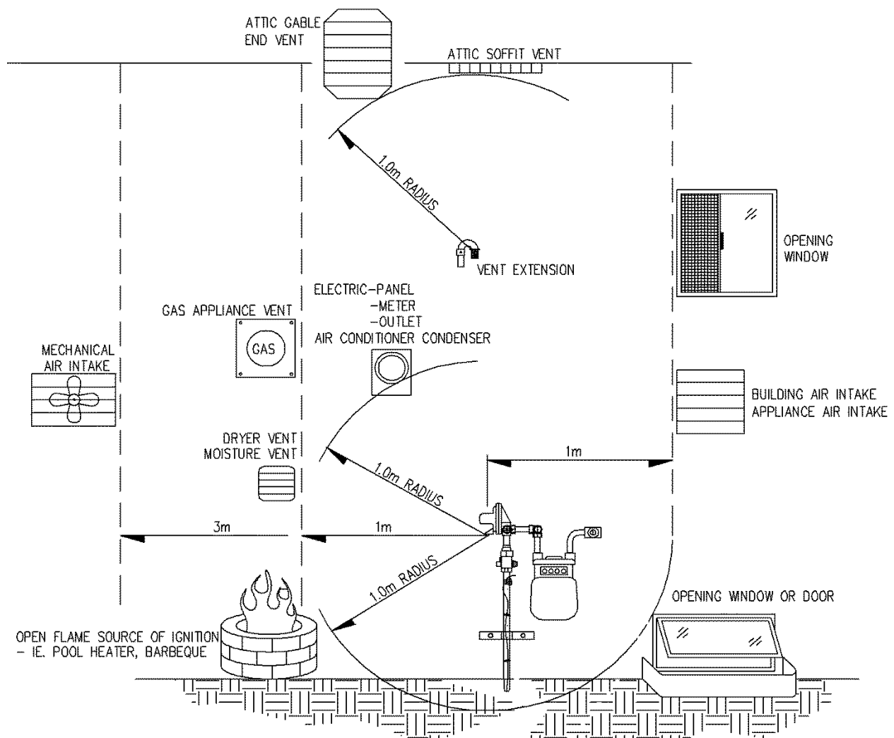
Figure 12 Separation Requirements for gas service
