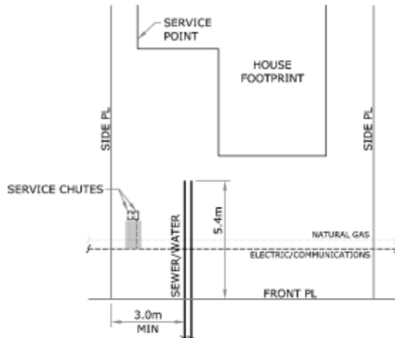
FIGURE 22 - TYPICAL SERVICE STUB LOCATION MAIN TRENCH ON EASEMENT
