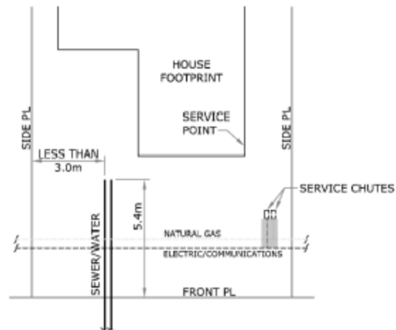
FIGURE 24 - ALTERNATE SERVICE STUB LOCATION MAIN TRENCH ON EASEMENT
