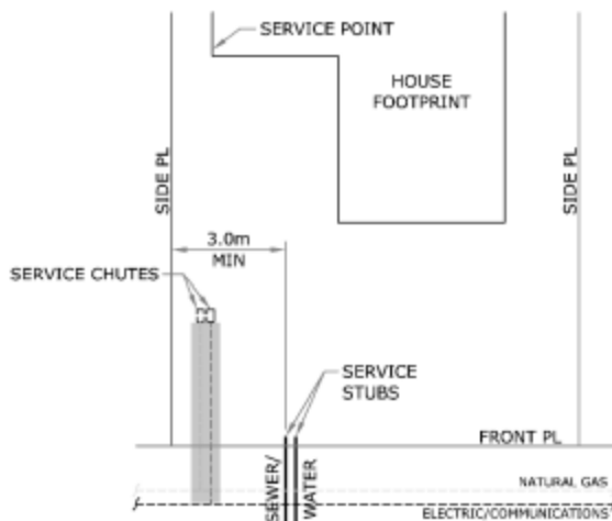
FIGURE 26 - TYPICAL SERVICE STUB LOCATION MAIN TRENCH ON RIGHT OF WAY
