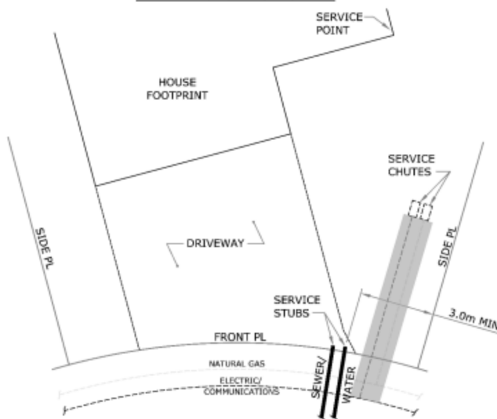
FIGURE 27 - TYPICAL SERVICE STUB LOCATION - PIE LOT MAIN TRENCH ON RIGHT OF WAY
